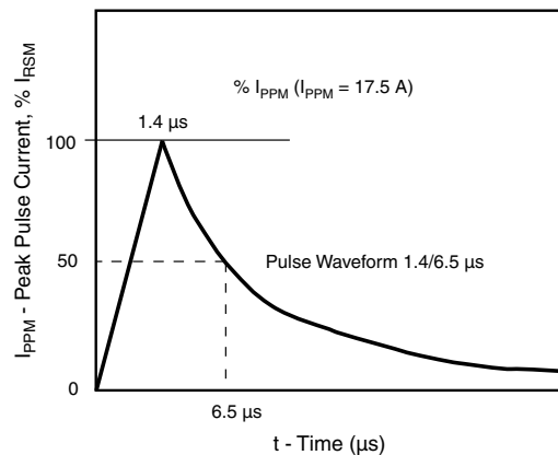
Fig. 2 - Pulse Waveform
